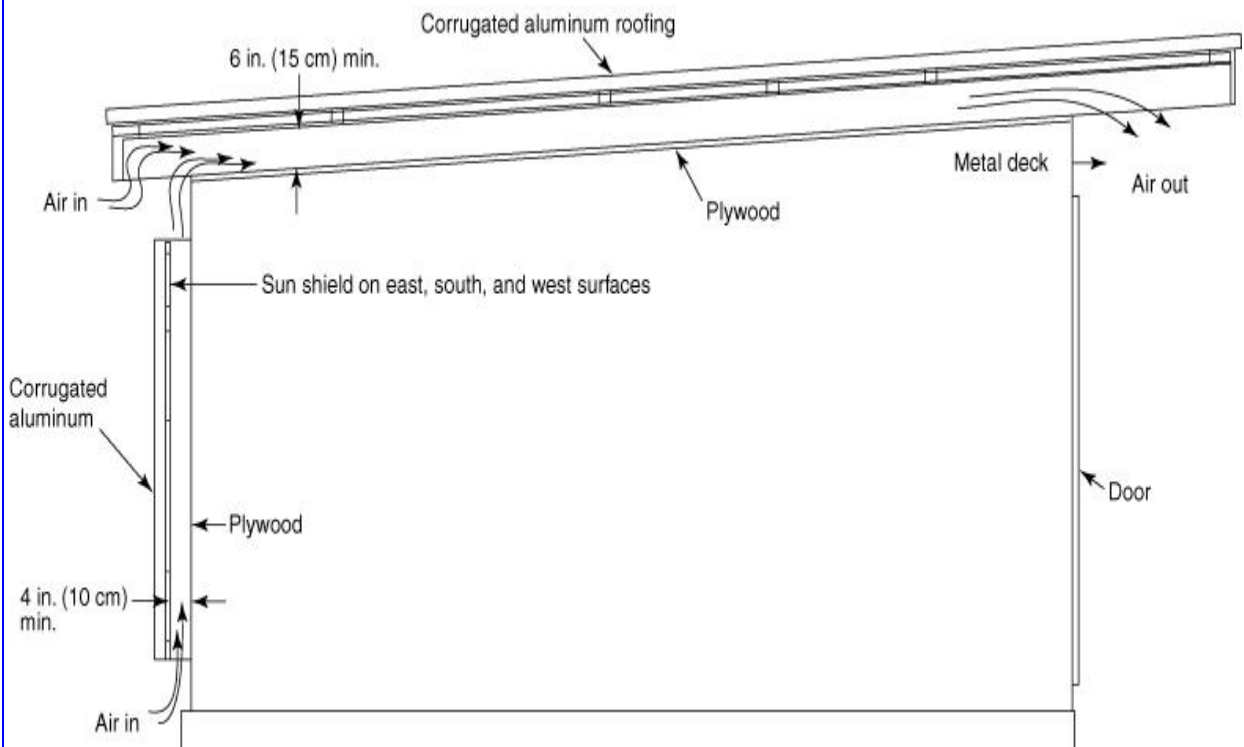
FIGURE A.7.4.3 Detached Storage Building for Storing Less than 5000 lb (2270 kg) of Organic Peroxide Formulations.
