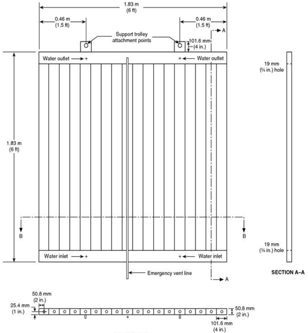
FIGURE A.5.3.1.1 Radiation Shield.
