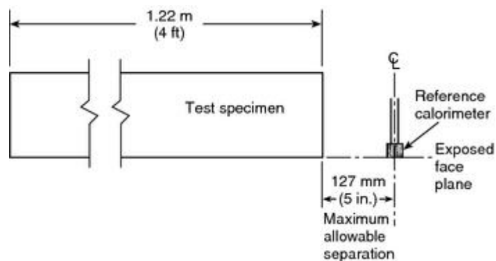
FIGURE 6.1.1.1 Plan View of Reference Calorimeter Location.
