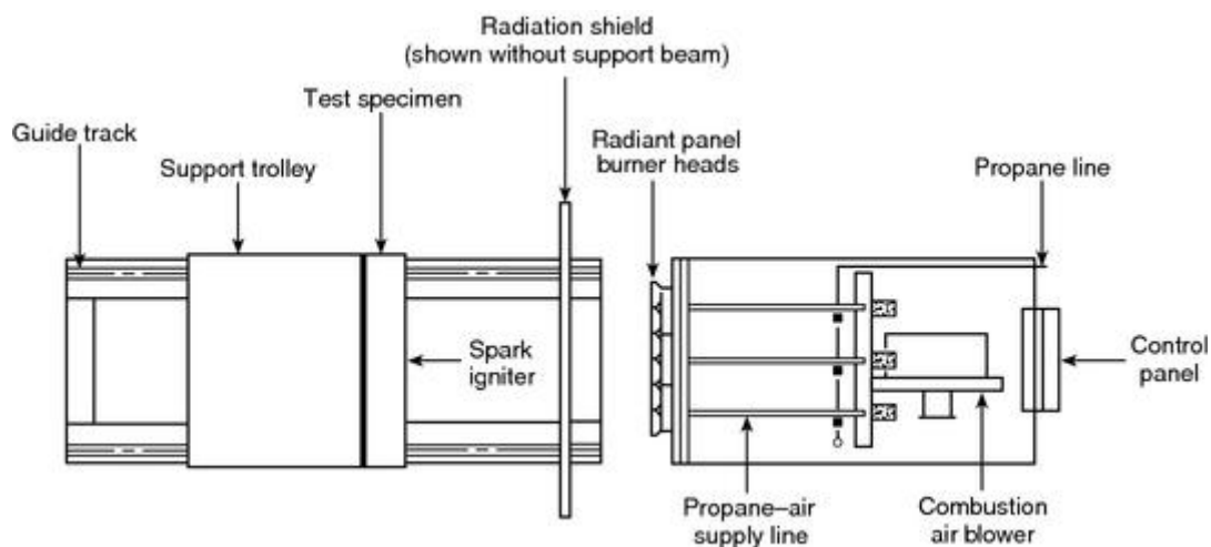
FIGURE 5.1.5(a) Plan View of the Test Apparatus.
