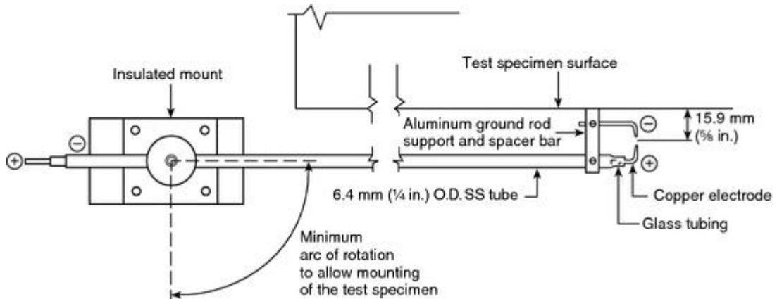
FIGURE 5.4.2.1(a) Plan View of the Spark Igniter.
