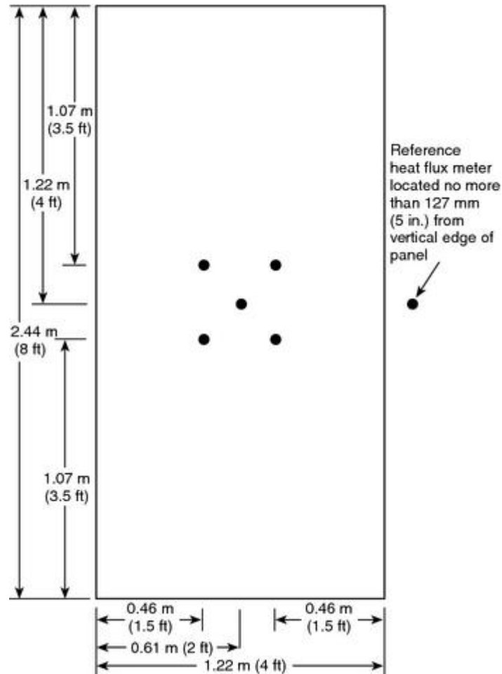
FIGURE 6.1.2 Calibration Panel Heat Flux Meter Locations.
