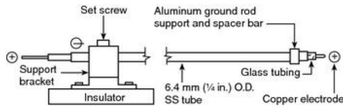
FIGURE 5.4.2.1(b) Side Elevation of the Spark Igniter.
