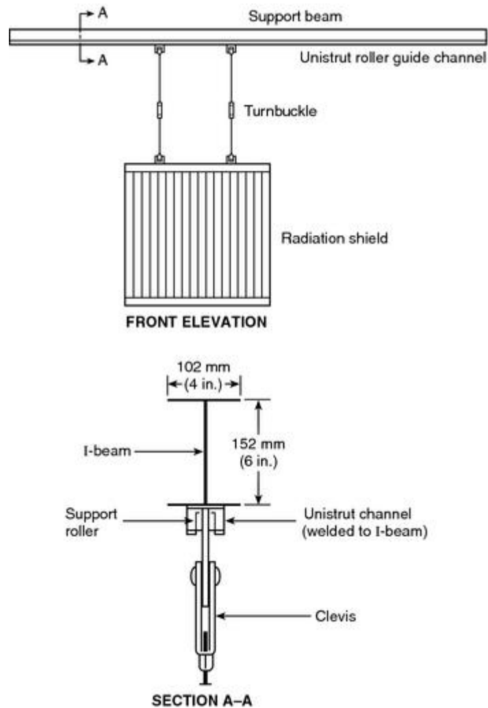
FIGURE A.5.3.3 Radiation Shield Support Trolley.
