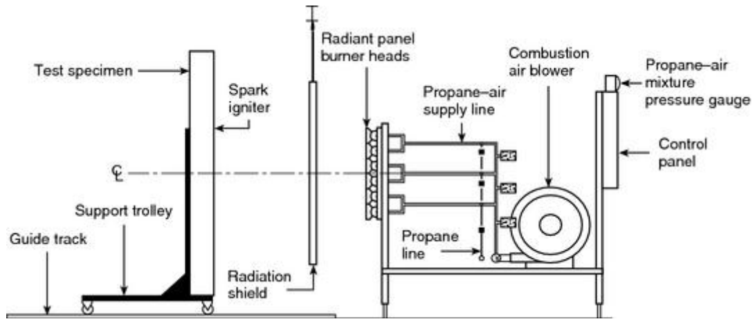
FIGURE 5.1.5(b) Side Elevation of the Test Apparatus.
