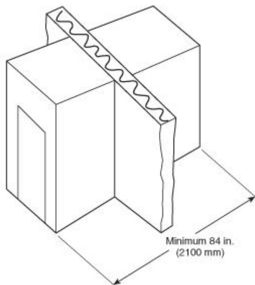
FIGURE A.5.8.3(a) Swinging Door and Sliding Door Configuration for Egress Purposes in an HC Fire Wall.
