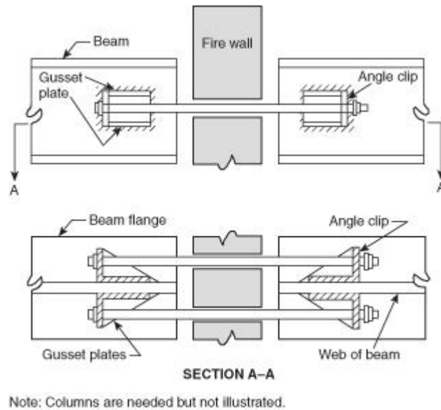
FIGURE A.5.4(f) Through-Wall Tie — Primary Roof Framing Perpendicular to Wall.
