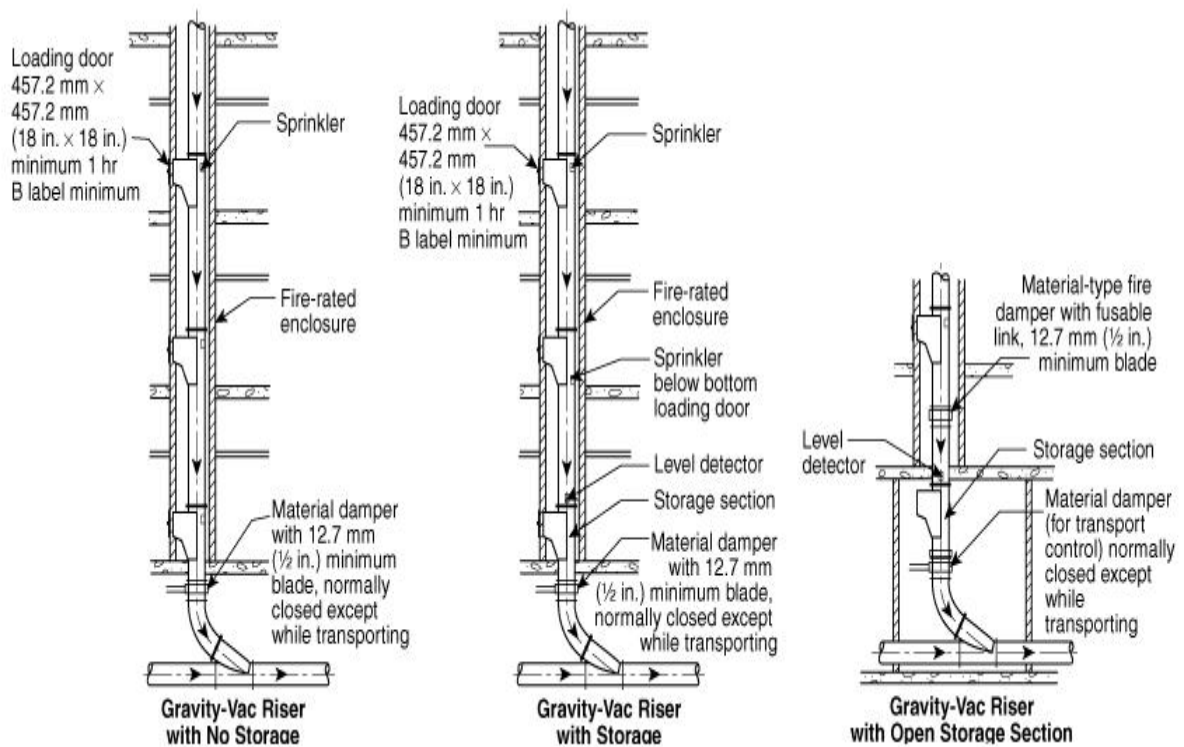
FIGURE A.5.4 Gravity Pneumatic System.
