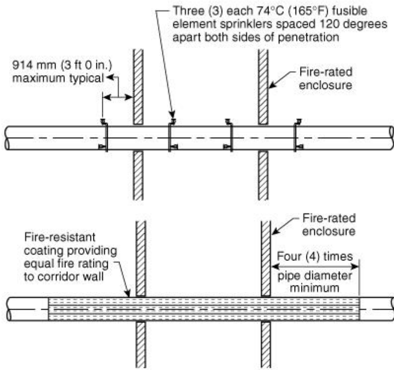
FIGURE A.5.3(c) Fire Damper Engineering Alternative for Penetration of Fire-Rated Enclosure.
