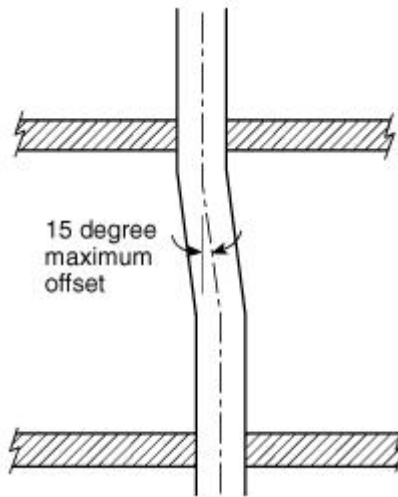
FIGURE 5.2.2.2 Gravity Metal Chute, Maximum Offset.
