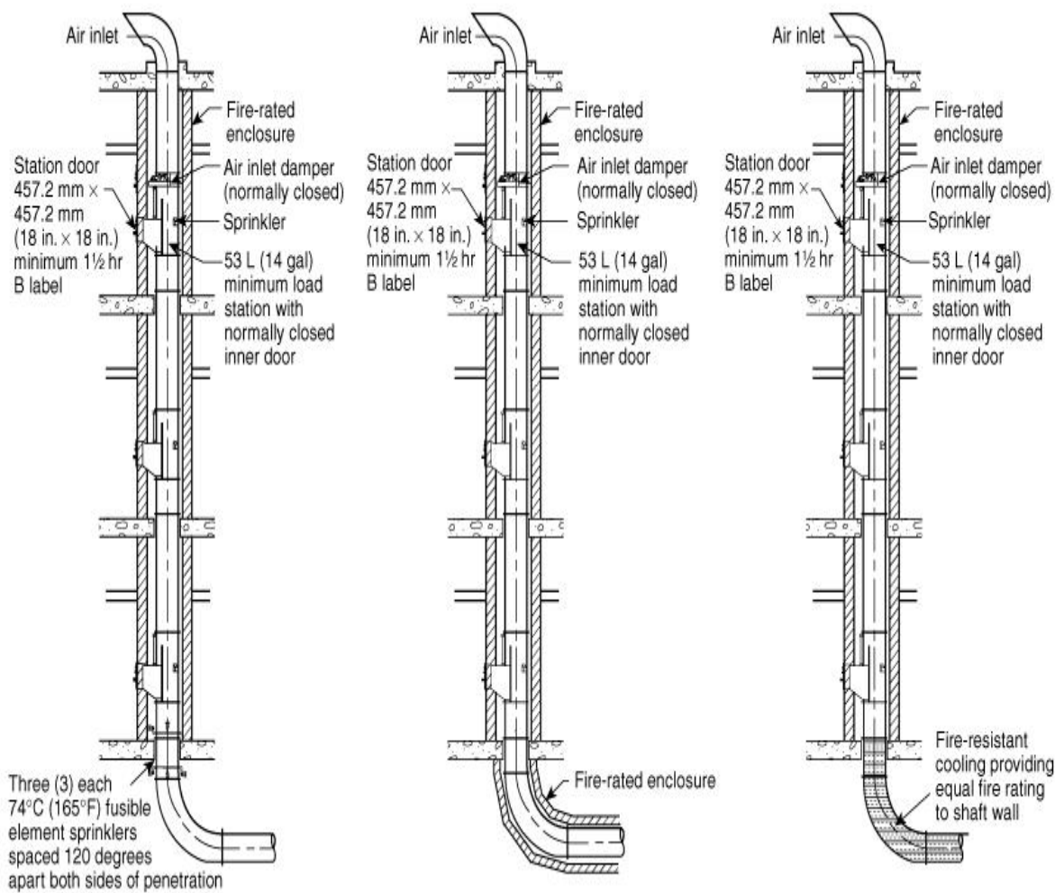
FIGURE A.5.3(b) Fire Damper Engineering Alternative for Penetration of Floor at Base of Shaft.
