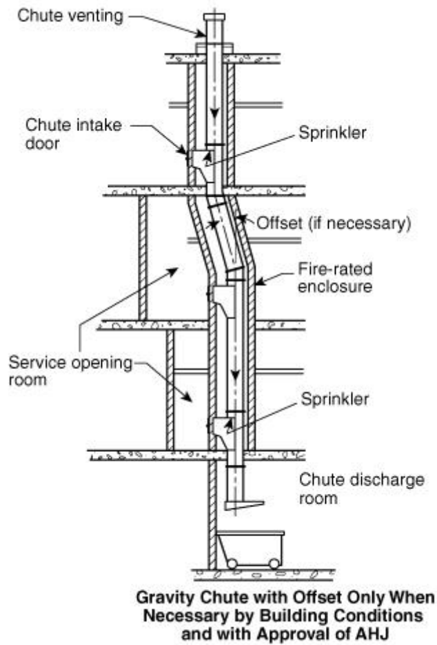
FIGURE A.5.2(b) Gravity Waste Chute.
