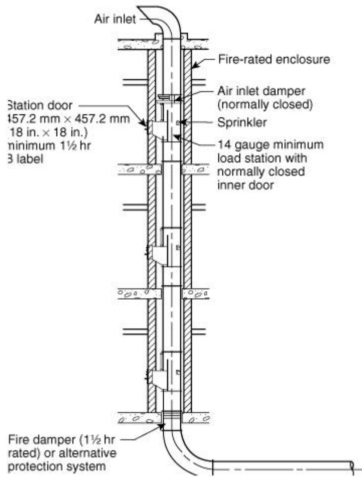
FIGURE A.5.3(a) Full Pneumatic System.
