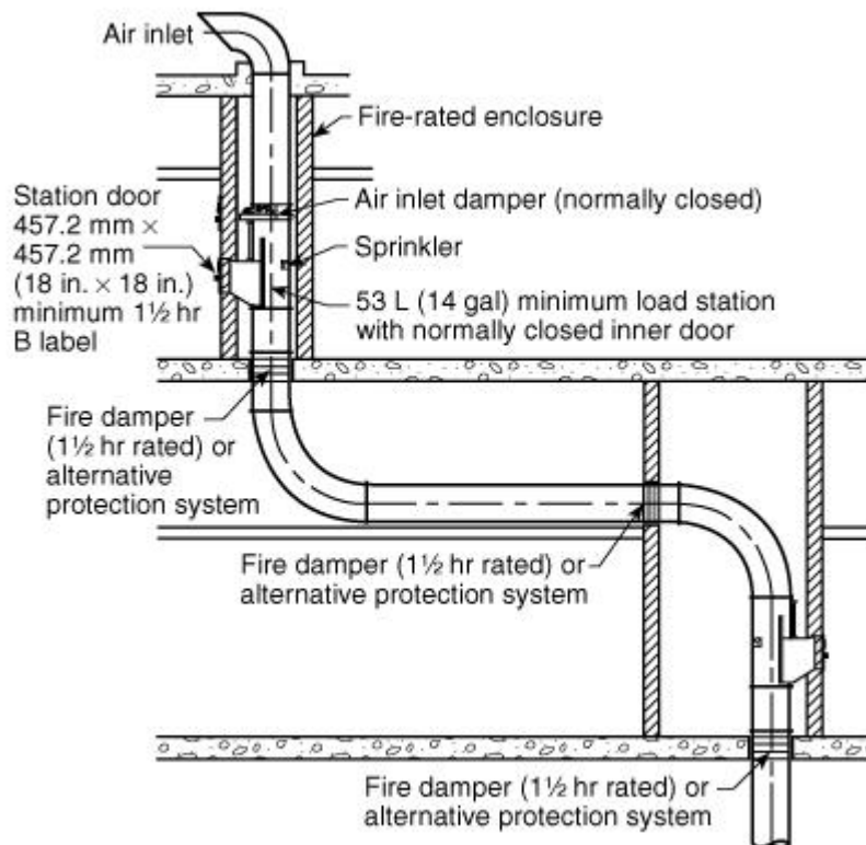
FIGURE 5.3.5.2.1(a) Full Pneumatic Riser with Offset.
