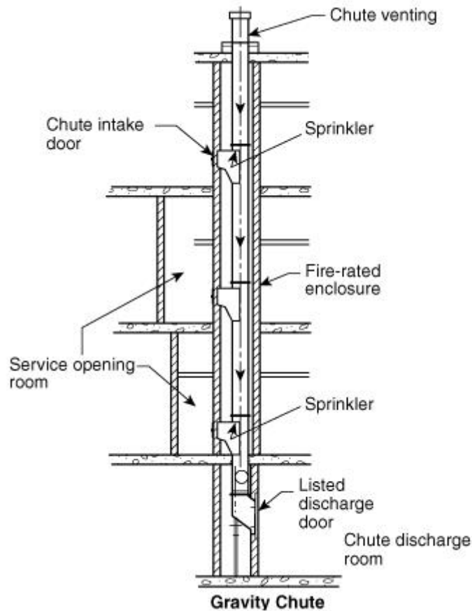
FIGURE A.5.2(a) Gravity Linen Chute.
